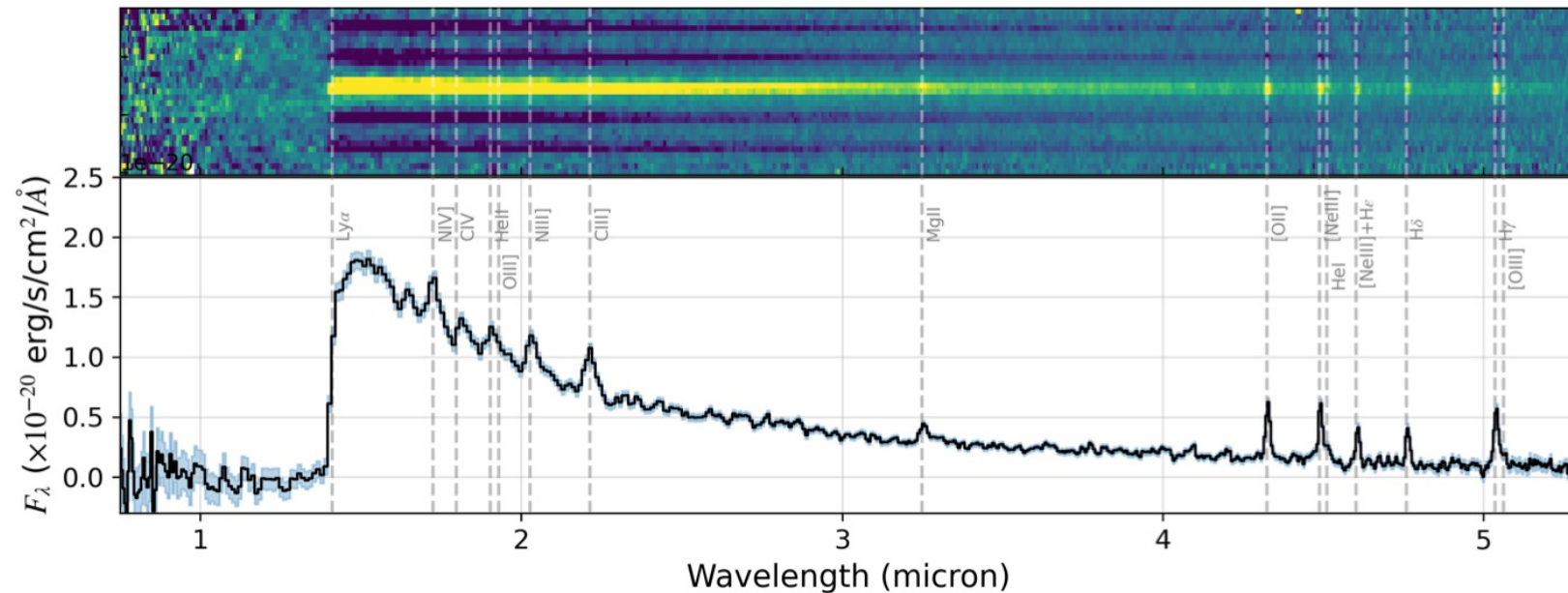
Fig. 1. 2D (top) and 1D (bottom) spectra of GN-z11 using PRISM/CLEAR configuration of NIRSspec. Prominent emission lines present in the spectra are marked. The signal to noise ratio (SNR) of the continuum is high and the emission lines are clearly seen in both the 1D and 2D spectra.
